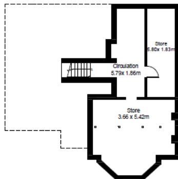
Basement Floor
